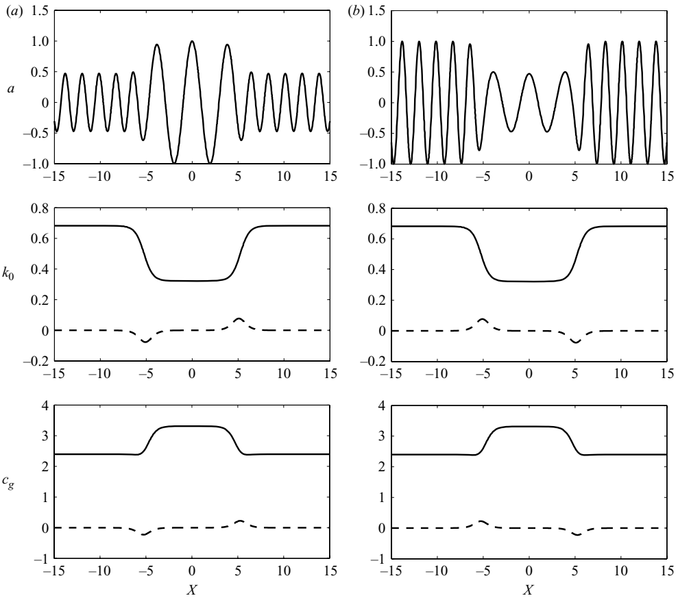
FIGURE 7. An example of (a) upstream and (b) downstream convective growth in a flow that is free of absolutely instability. The parameters are: (a) \delta = 0.2 , N_p = 2\delta , N_g = 0.4 ; (b) N_g = -0.4 .
